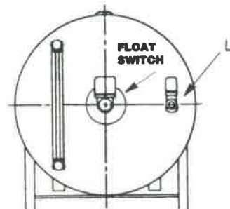
ELECTRIC SOLENOID MAKE-UP VALVE ASSEMBLY
